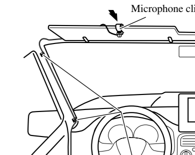
Microphone clip
