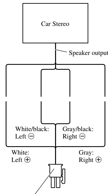
Speaker input connector To speaker input terminal of this unit.
