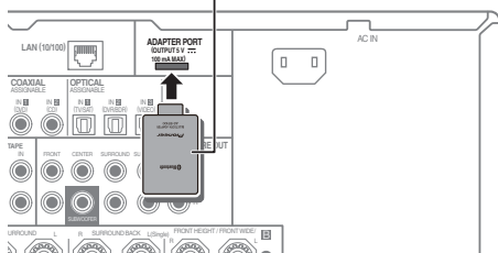
Bluetooth® ADAPTER (sold separately)
