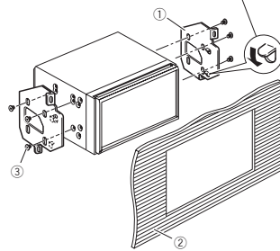
Truss head screw (5 mm × 8 mm) (6 pcs.)
